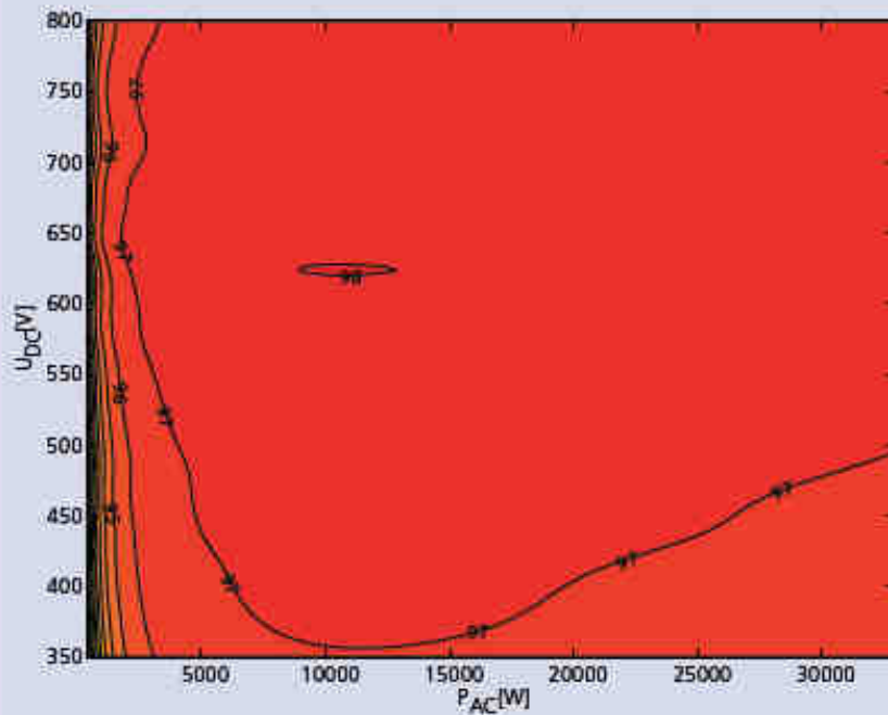
3D-Wirkungsgraddiagramm Powador 39.0 TL3
