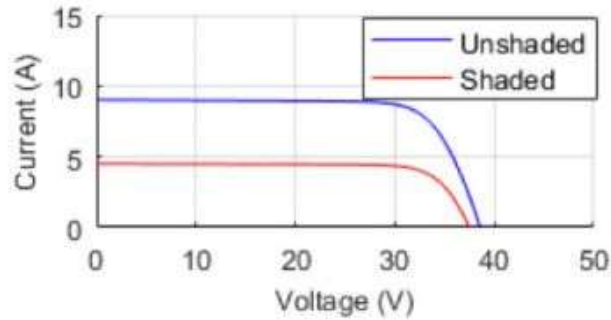
Standard Modules
